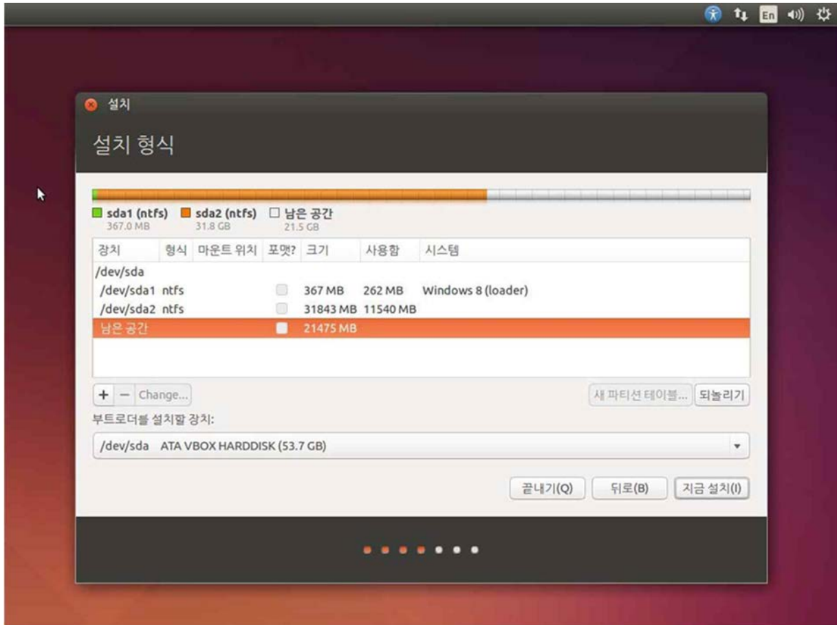
Figure 2 Installation Mode of Ubuntu 14.04 LTS
